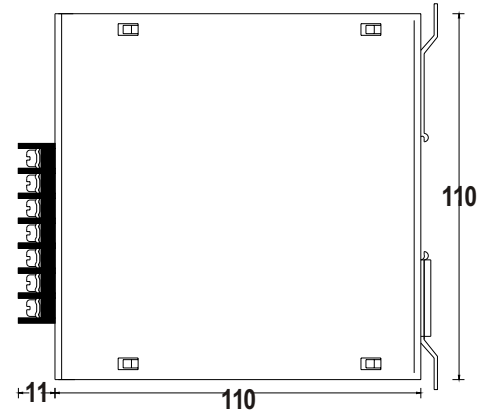
Dimensions:121(D)x110(H)x100(W)mm
