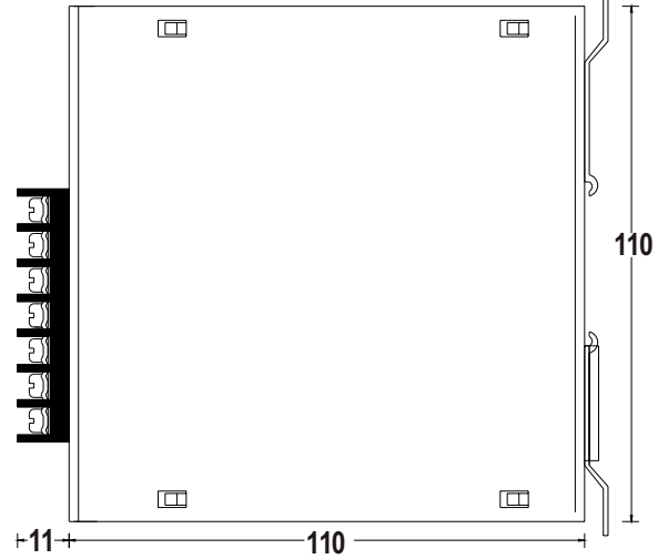
Dimensions: 121(D)x110(H)x40(W)mm
