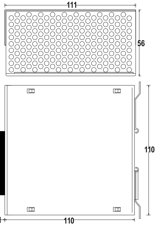
Dimensions: 121(D)x110(H)x56(W)mm
