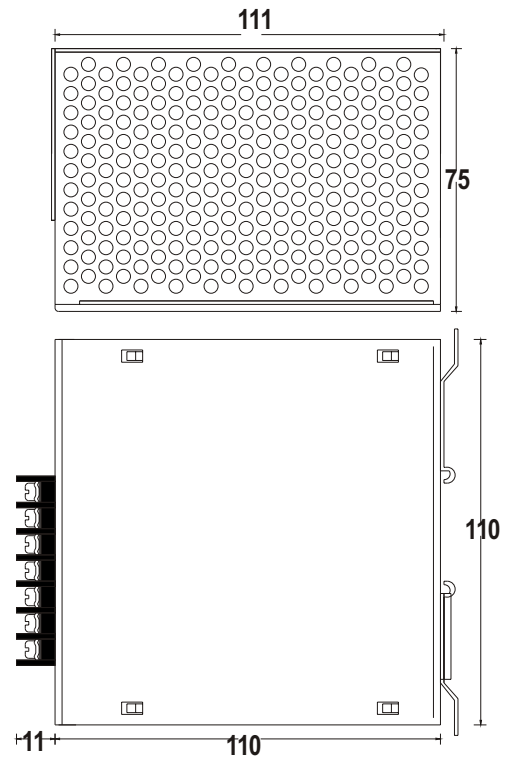
Dimensions: 121(D)x110(H)x75(W)mm
