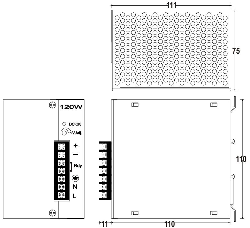
Dimensions:121(D)x110(H)x75(W)mm
